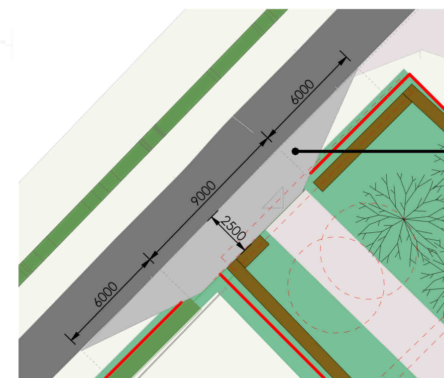
Proposed Lay-by 1 : 200
